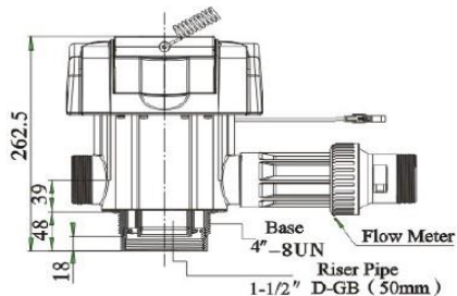
Structure Chart of F74B3 (63610B)
