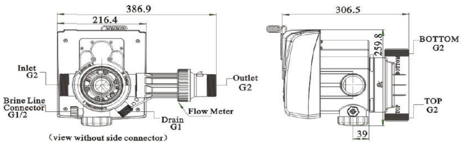
Structure Chart of N74A3 (63610)
