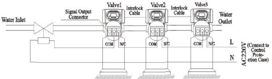
Figure 3-4 Wiring of Solenoid Valve in Inlet
