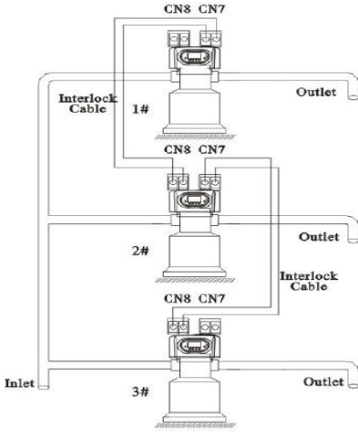
Figure 3-12 Interlock system
