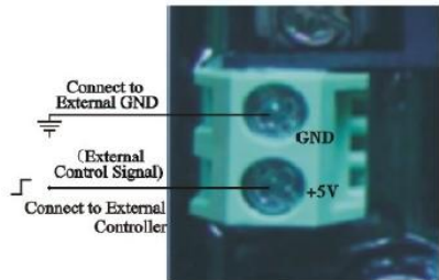
Figure 3-11 Wiring of Remote Input
